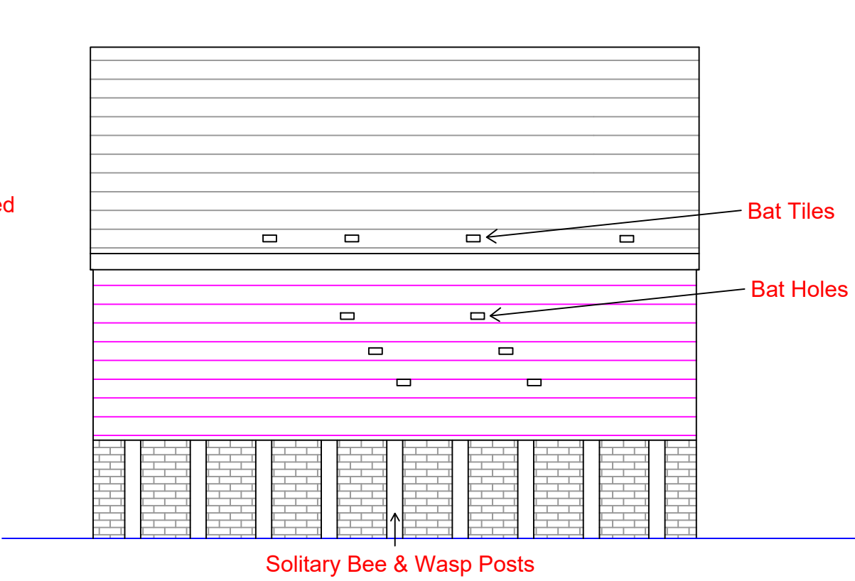
Proposed Front Elevation 1:50
