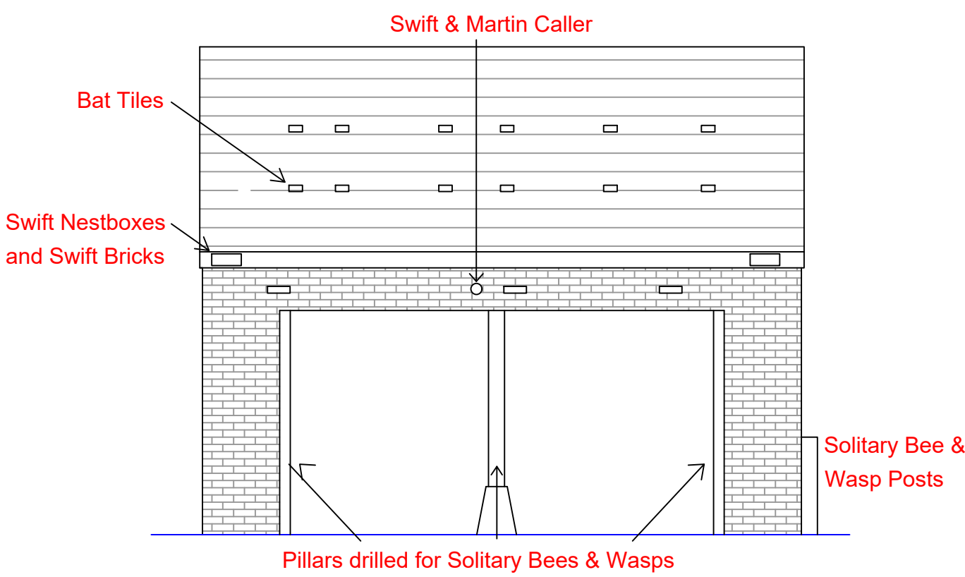
Proposed Front Elevation 1:50
