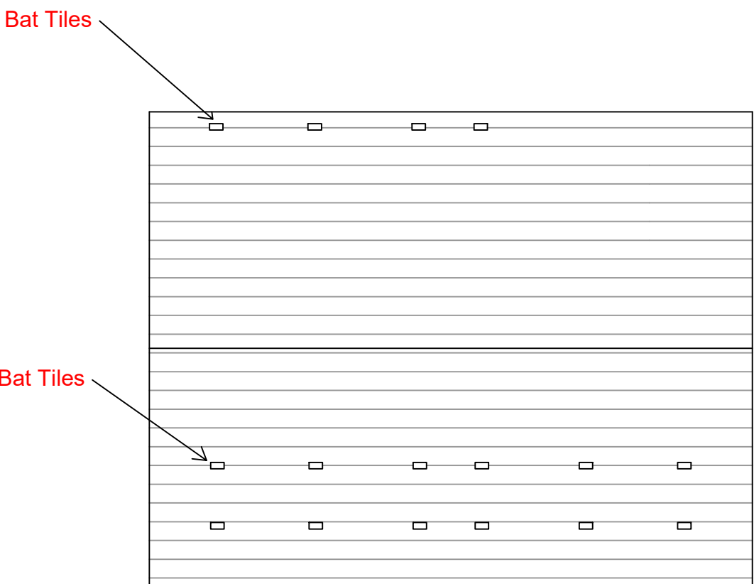
Proposed Roof Plan 1:50
