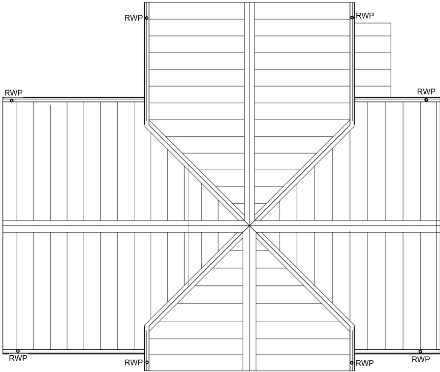
1 Proposed Roof Plan
