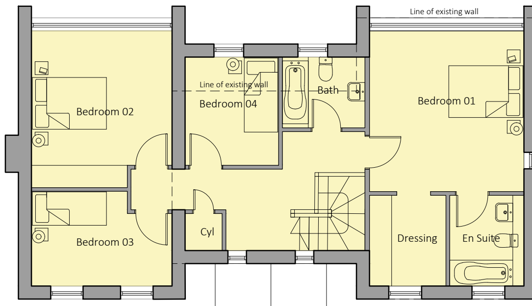
First Floor Plan GIA 82.5M2
