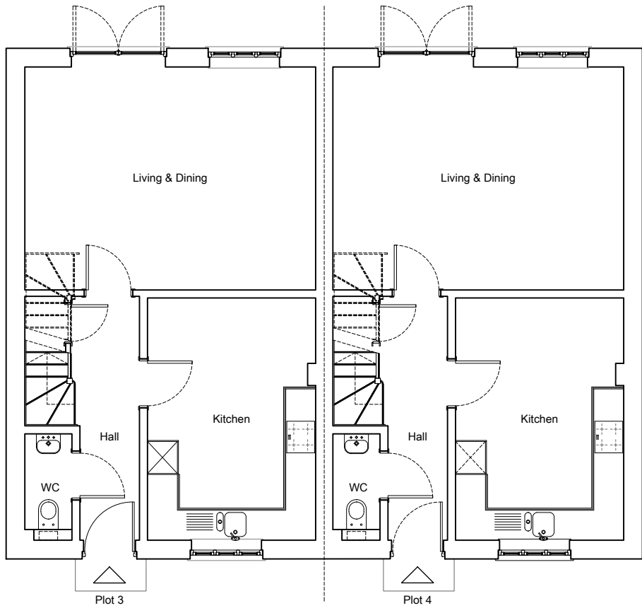
Ground Floor Plan - Plots 3 & 4 Proposed
