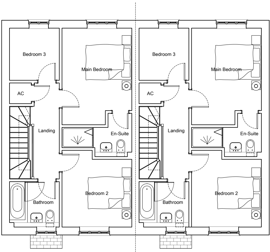
First Floor Plan - Plots 3 & 4 Proposed
