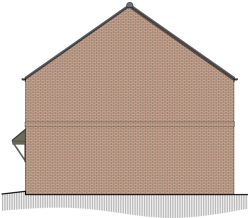
Side Elevation - Plots 3 & 4 Proposed
