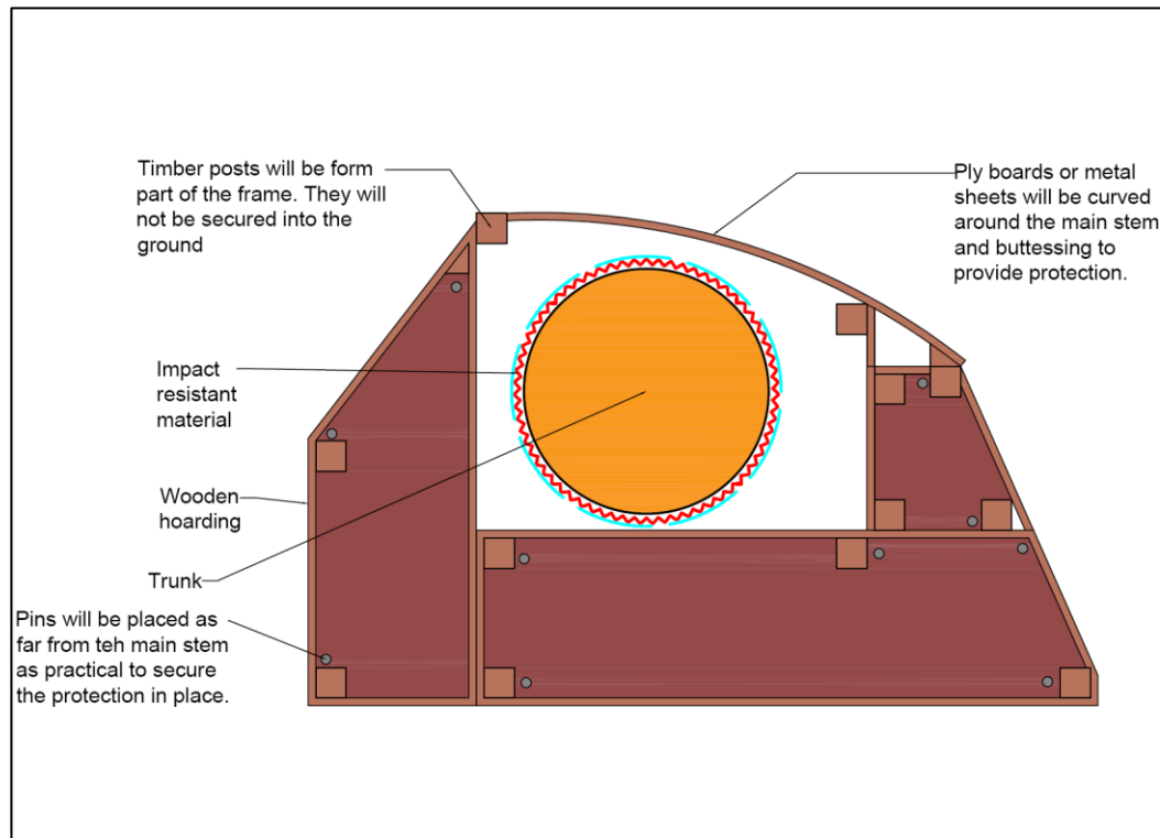
Figure 5 – Indicative example of a curved tree protection barrier from viewed from side
