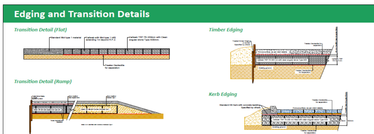
Figure 7 – Cellweb edging and transition details
