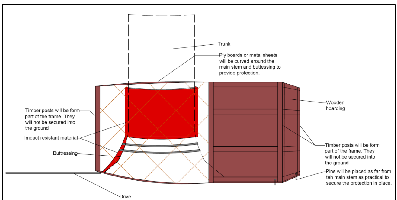
Figure 5 – Indicative example of a curved tree protection barrier from viewed from side
