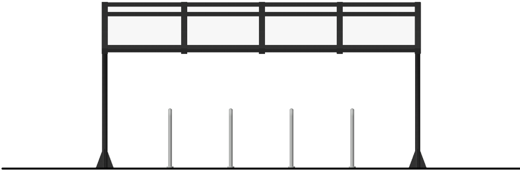
PROP. BIKE SHELTER ELEV 1:50 - REAR
