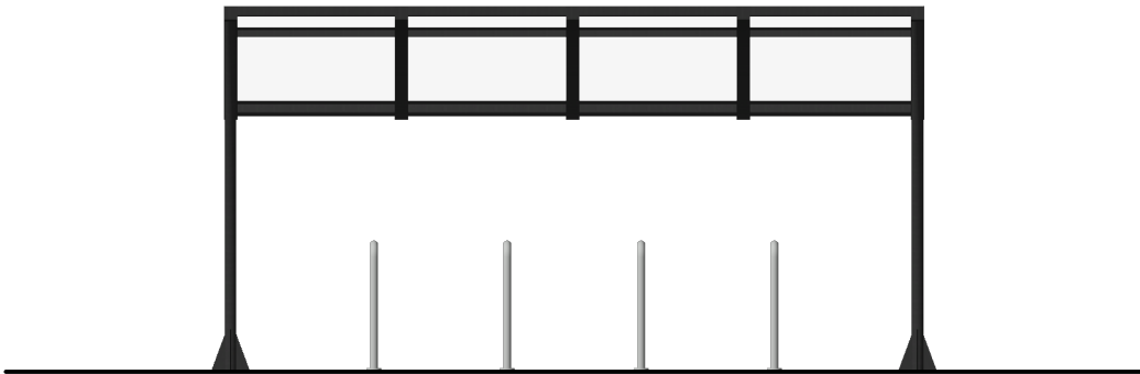
PROP. BIKE SHELTER ELEV 1:50 - FRONT
