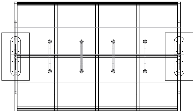
PROP. BIKE SHELTER PLAN 1:50
