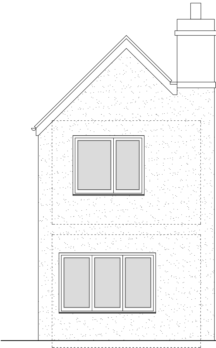
REAR ELEVATION (PARTIAL) - scale 1:50
