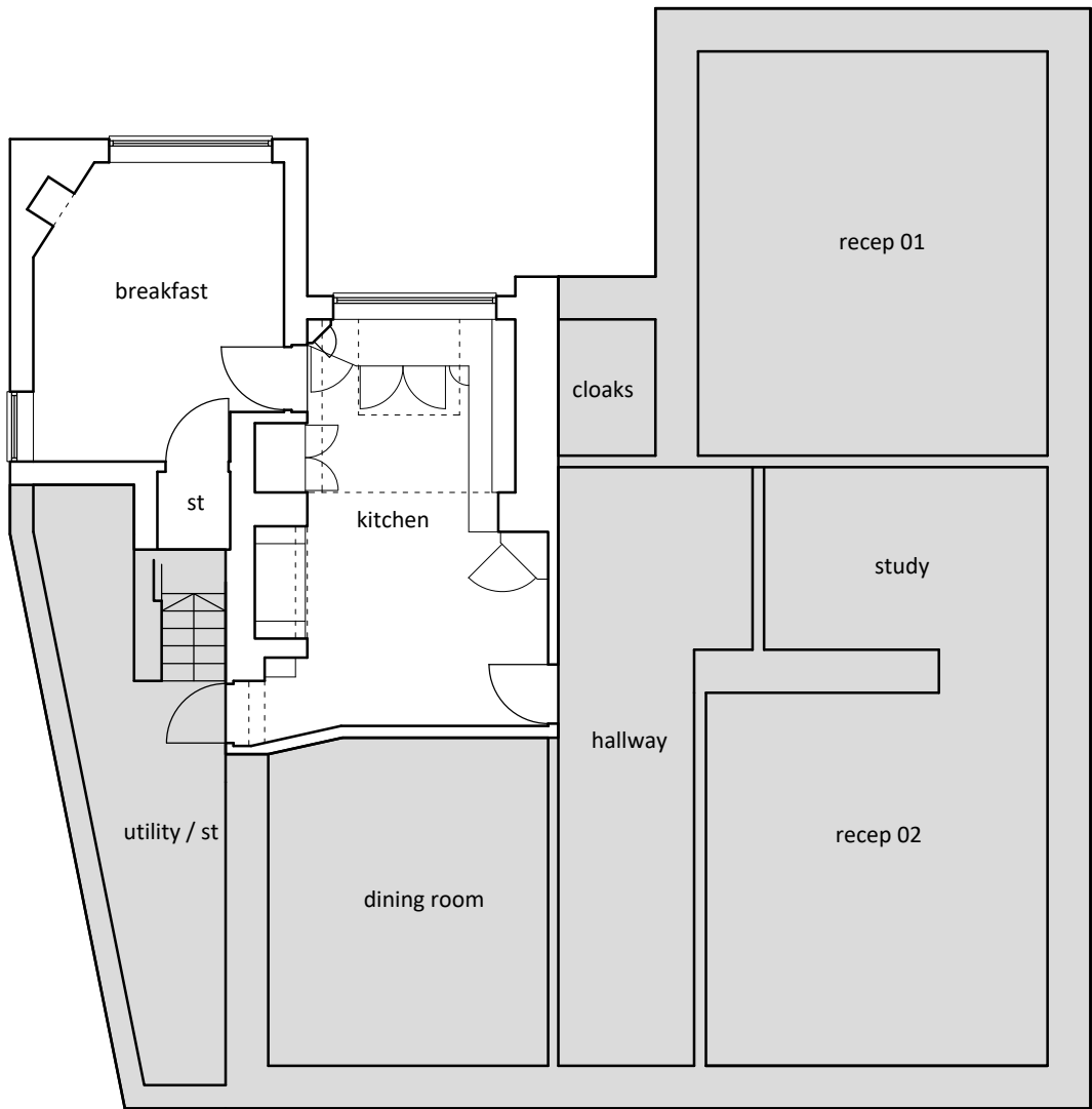
GROUND FLOOR (PARTIAL PLAN) - scale 1:100
