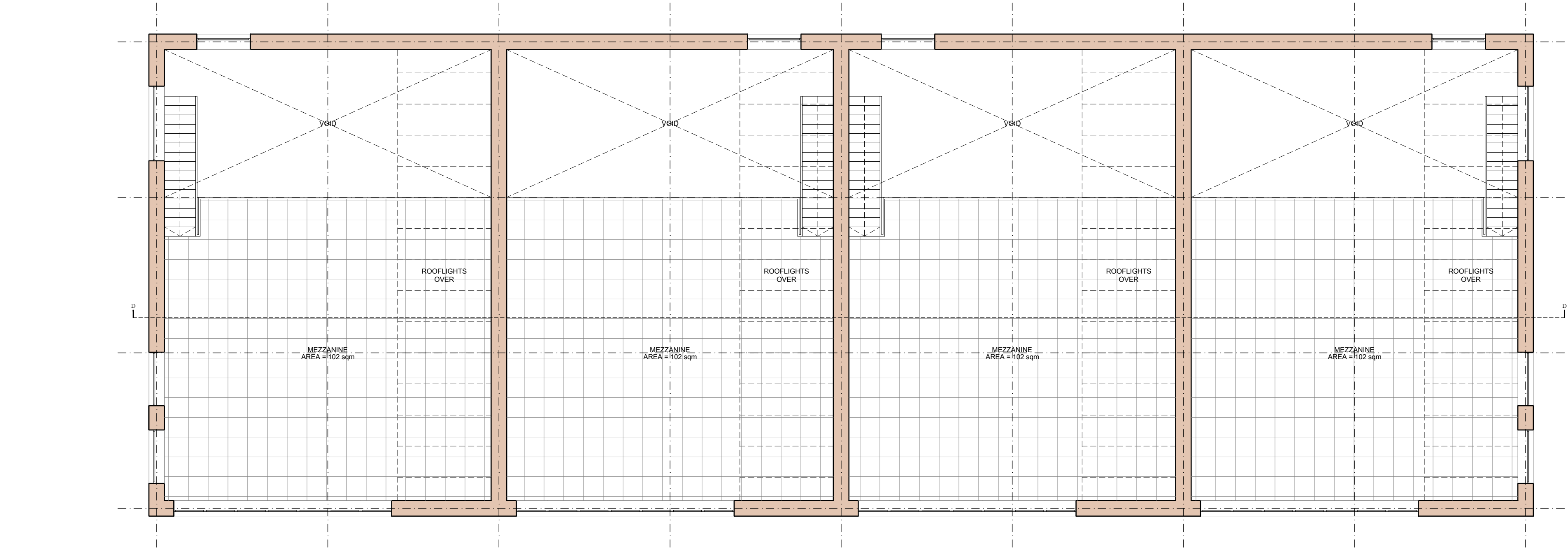
0 5m First Floor Plan - Block B Proposed
