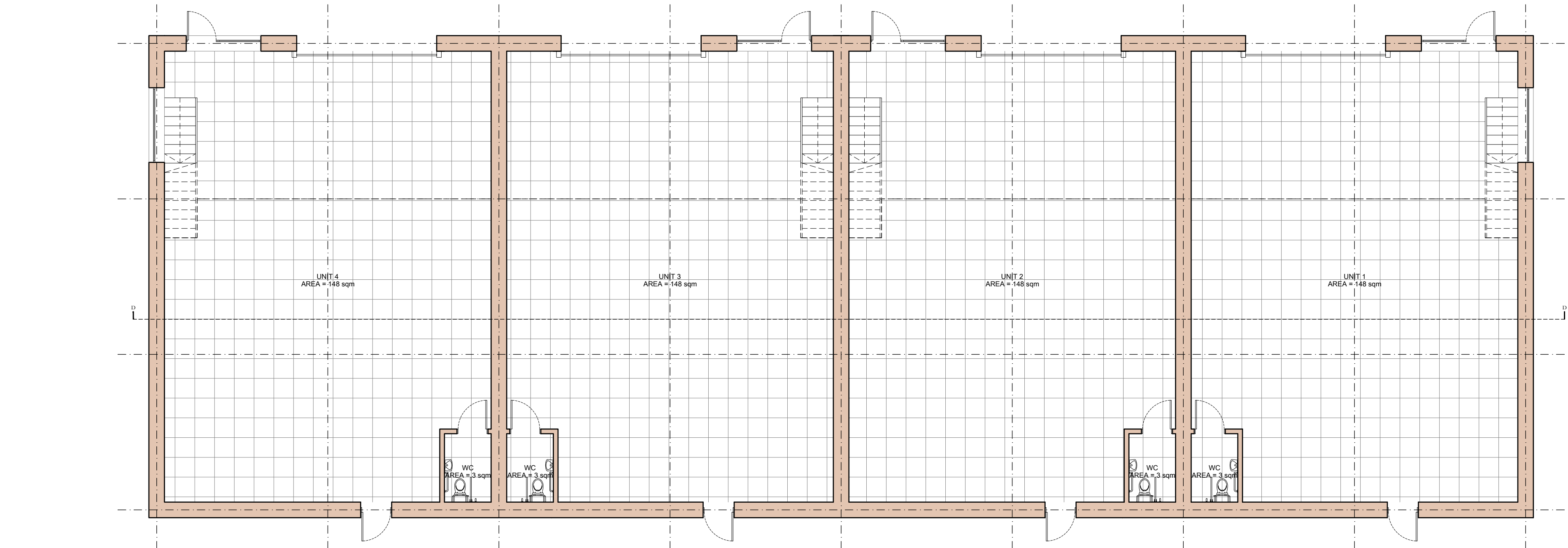
0 5m Ground Floor Plan - Block B Proposed
