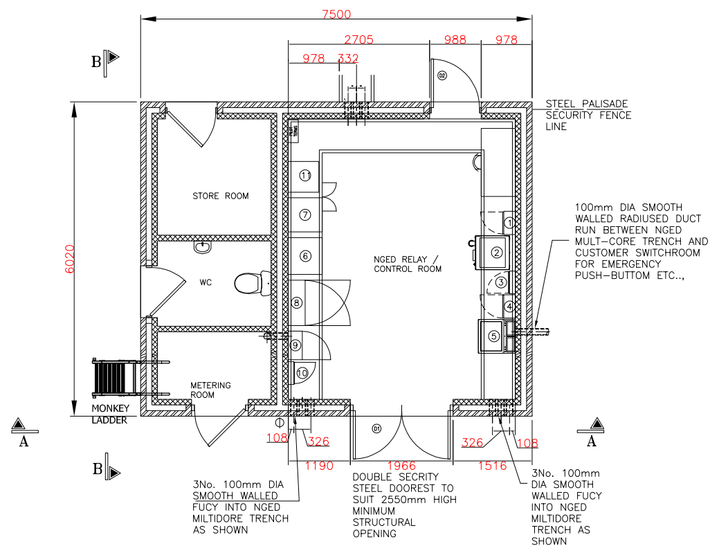
PLAN TOP VIEW OF DNO CONTROL STATION
