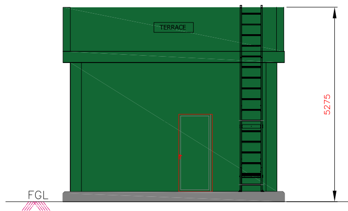
ELEVATION OF DNO CONTROL STATION
