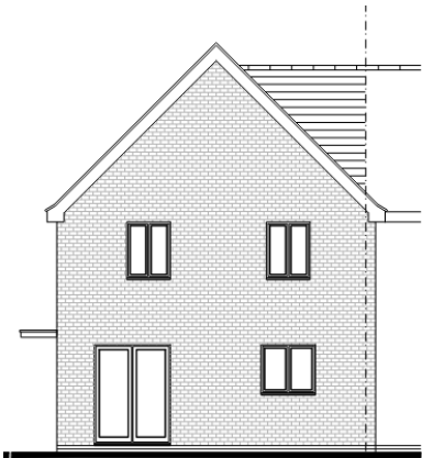
Rear Elevation Plot 15
