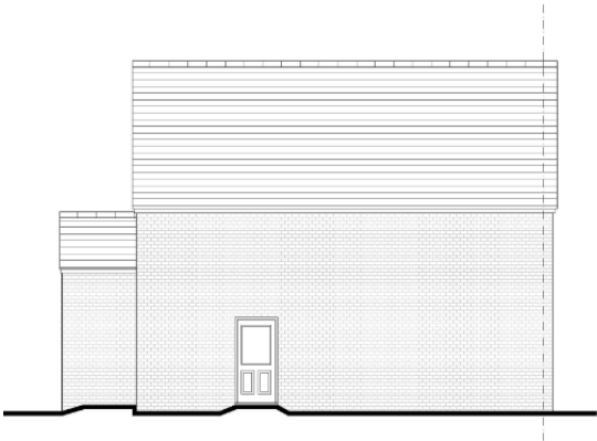
Rear Elevation Plot 9 & 10
