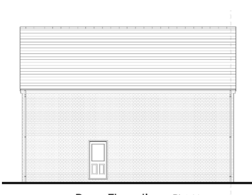
Rear Elevation Plot 11
