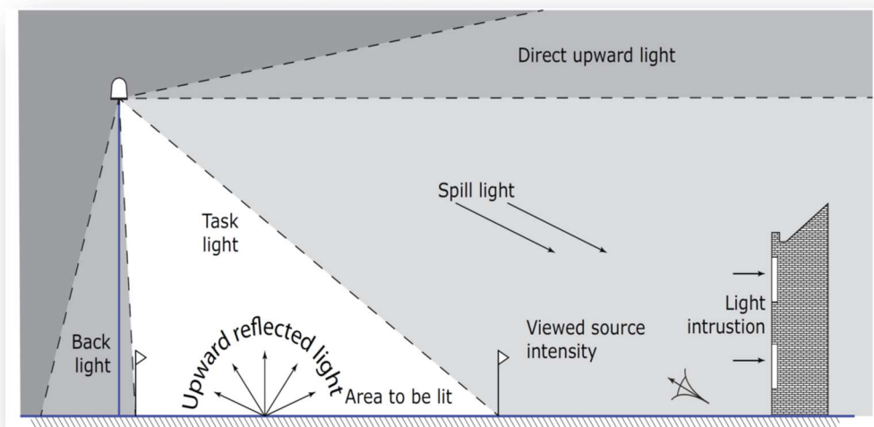
Figure 3.1: Obtrusive light diagram
