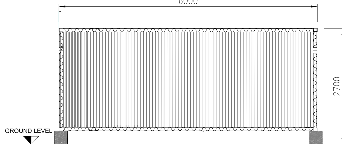
Side View
