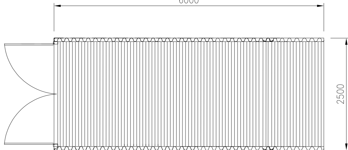
Top View
