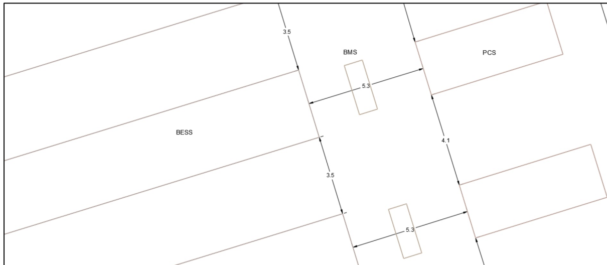
Figure 4 - BESS and PCS unit spacing.
