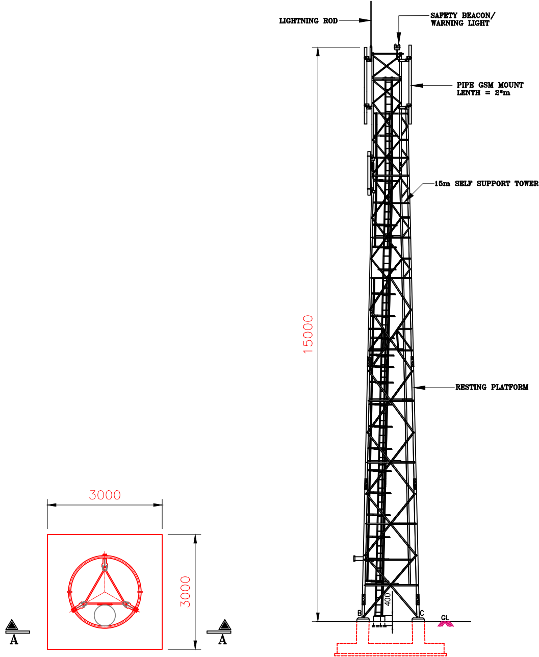
PLAN VIEW
