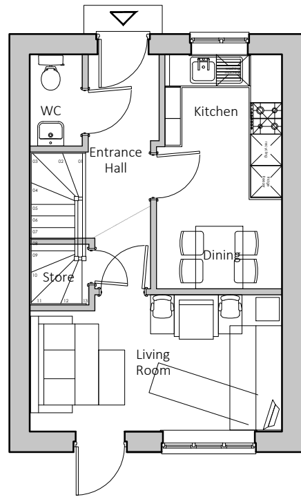
Ground Floor Plan 1:100@A3
