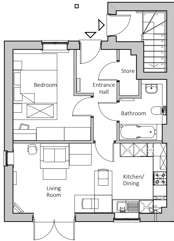
Ground Floor Plan 1:100@A3
