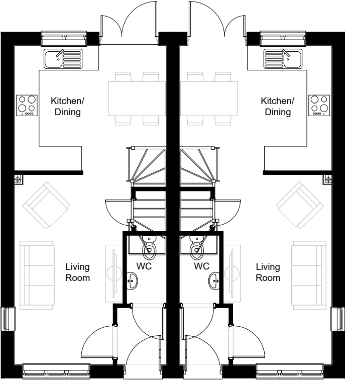
House Type A2 - Ground Floor Plan
