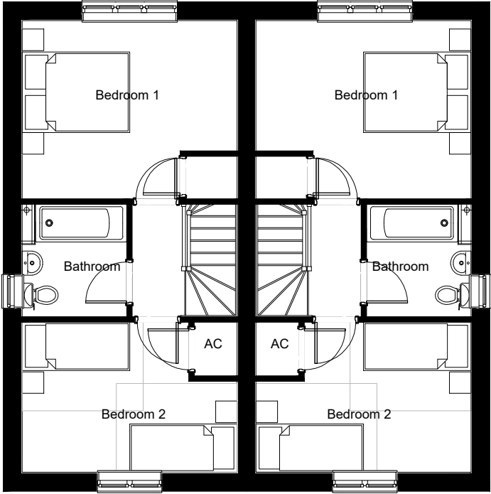
House Type A2 - First Floor Plan
