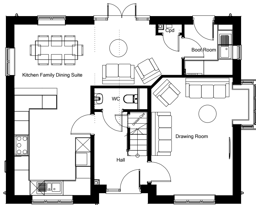
House Type DV1+ - Ground Floor Plan
