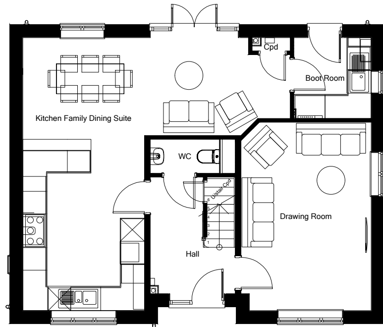
House Type DV1 - Ground Floor Plan
