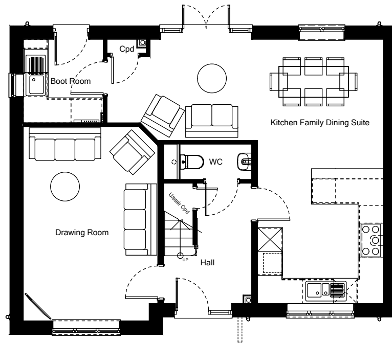
House Type D - Ground Floor Plan
