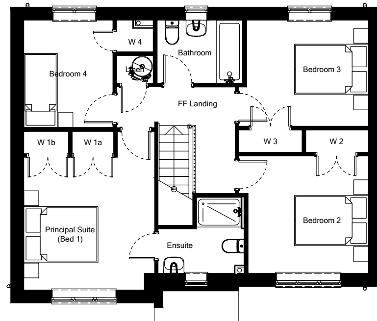
First Floor Plan - D Type
