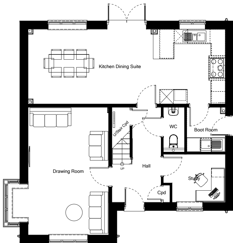
House Type P+ - Ground Floor Plan
