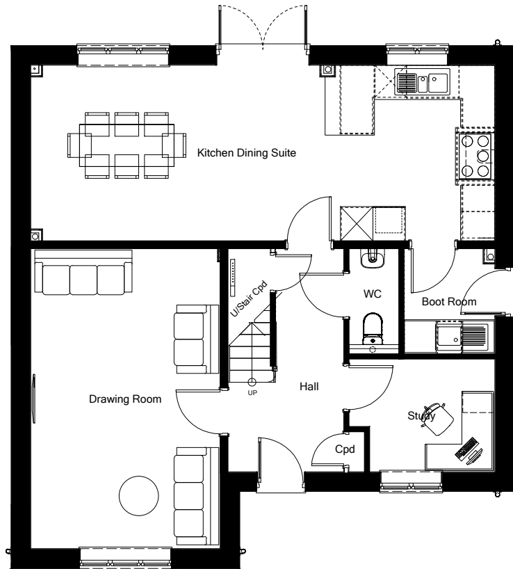
House Type P - Ground Floor Plan
