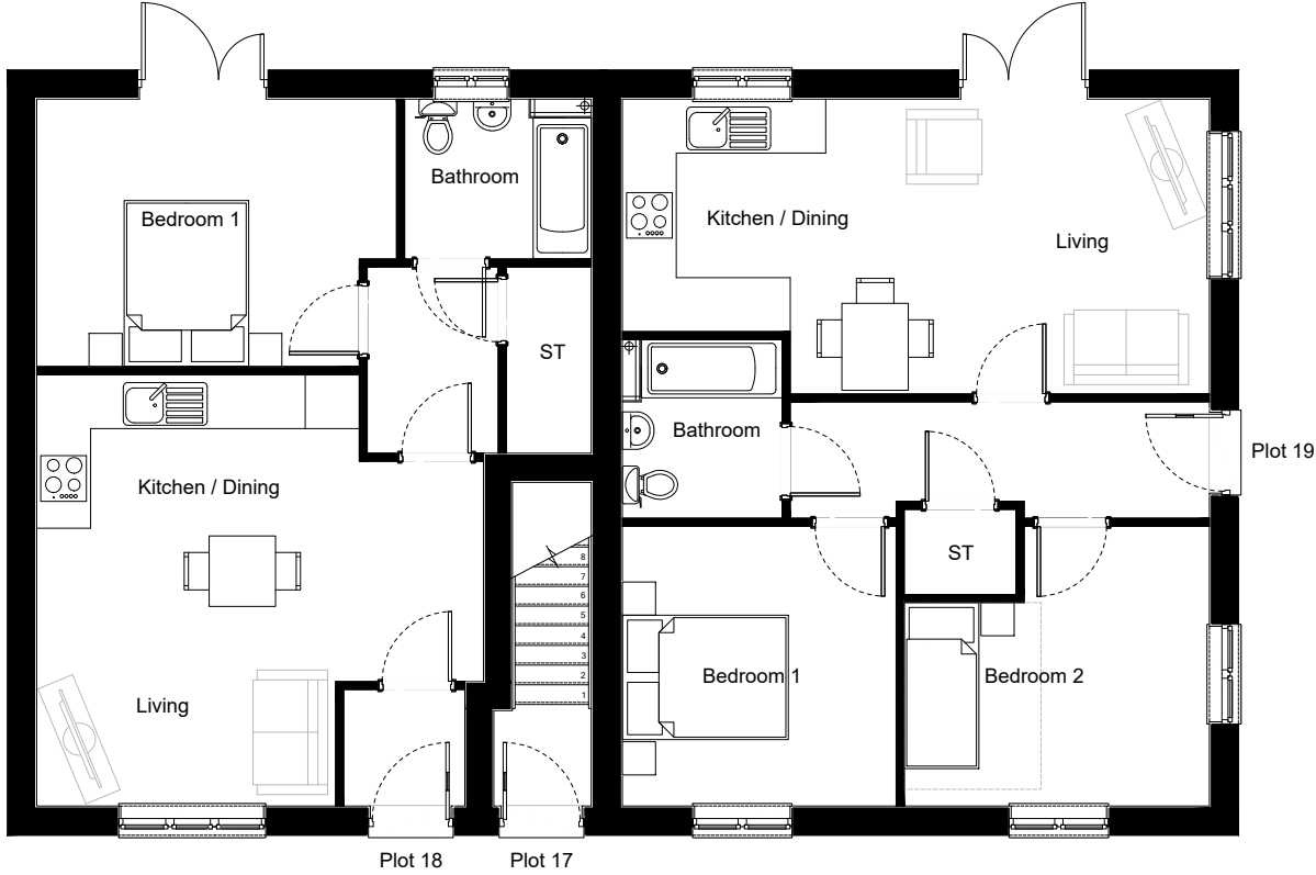
House Type A1M Ground Floor Plan
