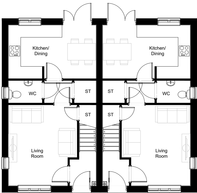
House Type A3 - Ground Floor Plan
