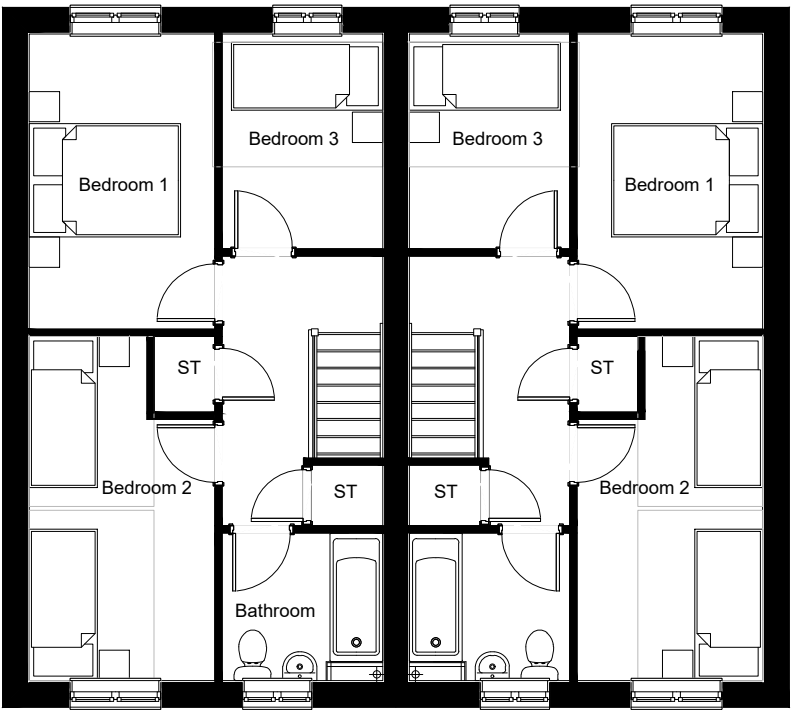
House Type A3 - First Floor Plan
