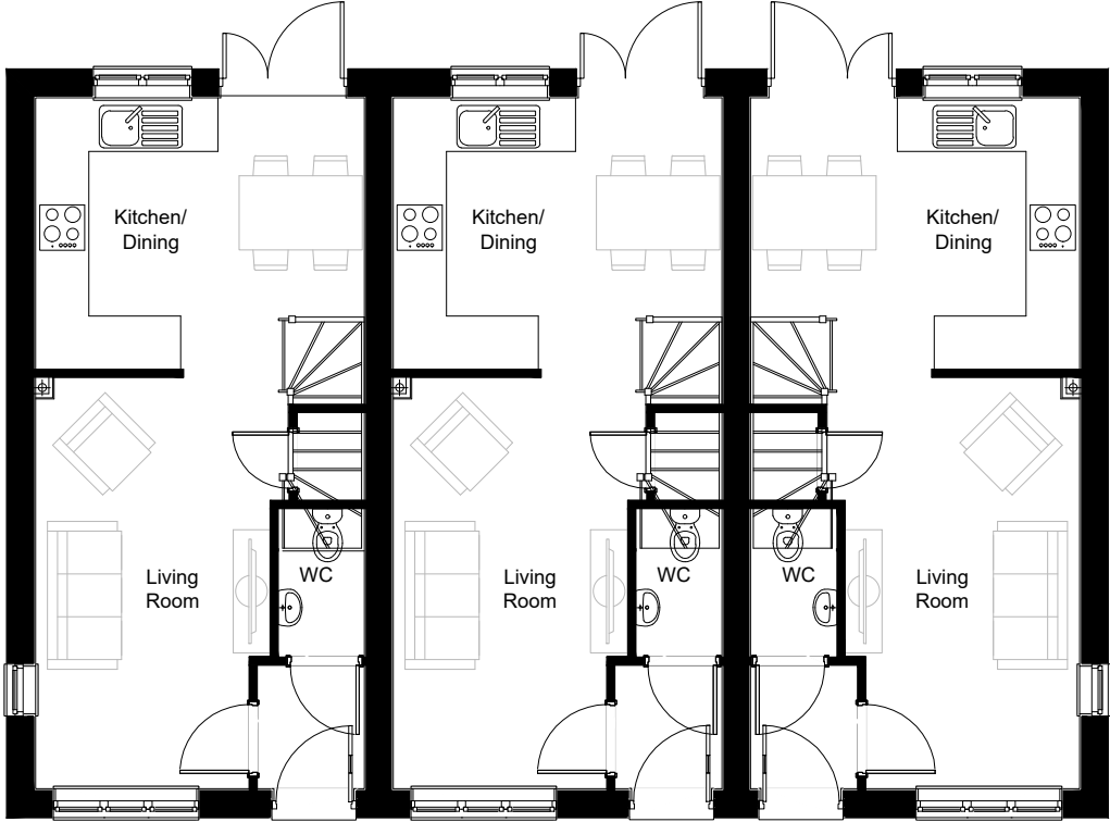
House Type A2 - Ground Floor Plan
