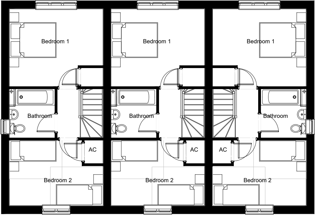
House Type A2 - First Floor Plan
