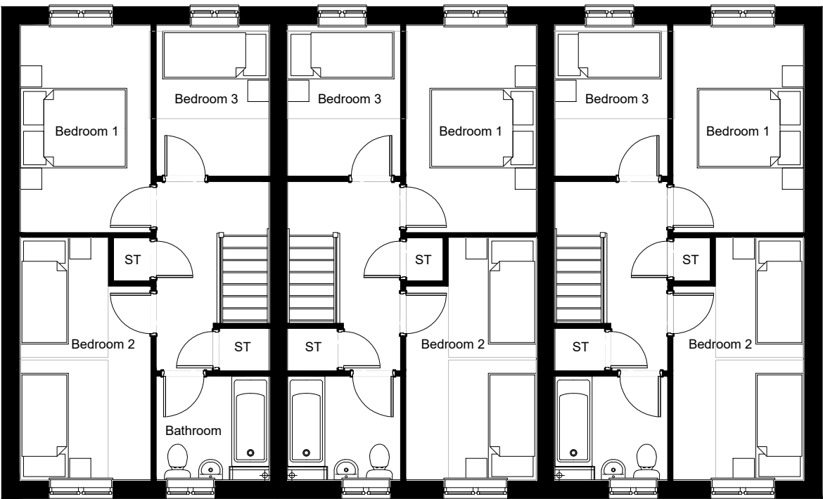
House Type A3 - First Floor Plan
