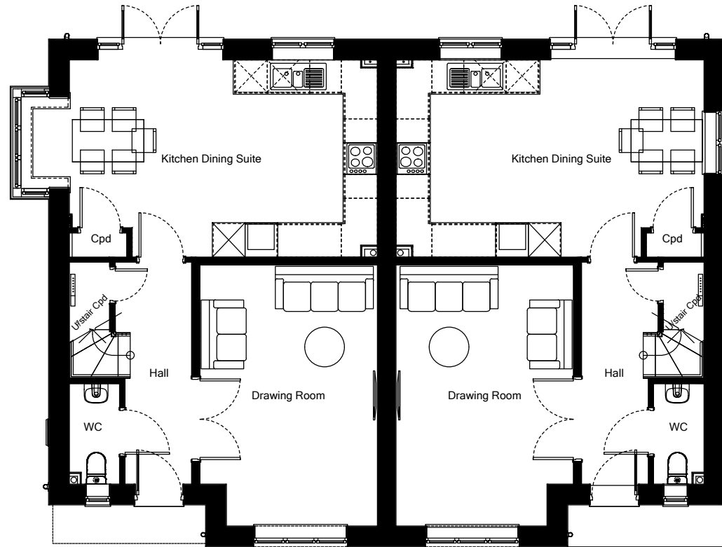
House Type M+ & M - Ground Floor Plan
