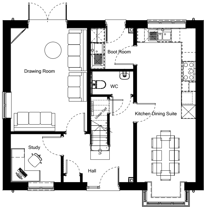
House Type B - Ground Floor Plan
