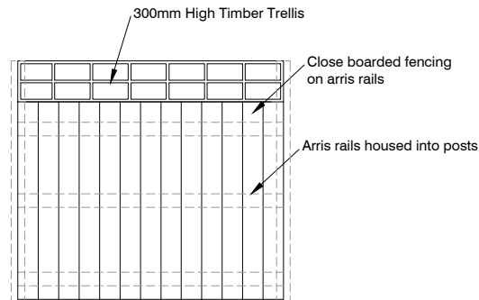
1.5m High Close Board Fence with 300mm Timber Trellis
