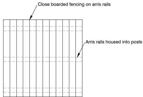
1.8m High Close Board Fence
