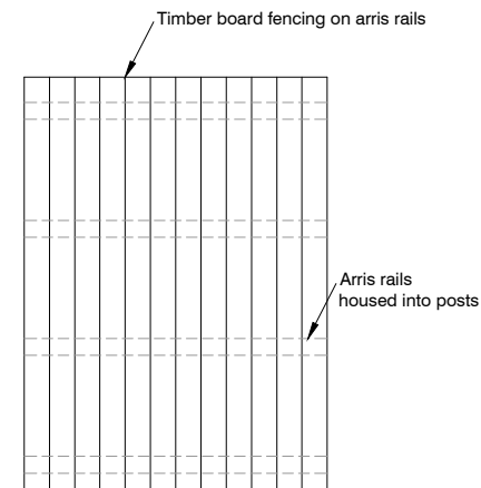
2.5m High Timber Acoustic Fence
