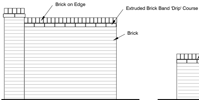
1.8m High Brick Screen Wall 2m High Brick Piers where shown
