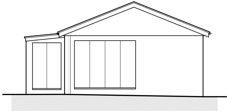
133.000m South East Elevations 1:100
