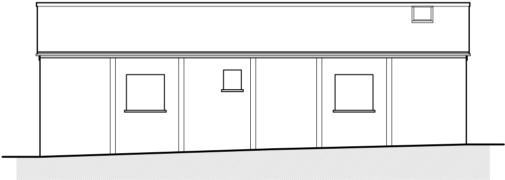
133.000m North East Elevations 1:100
