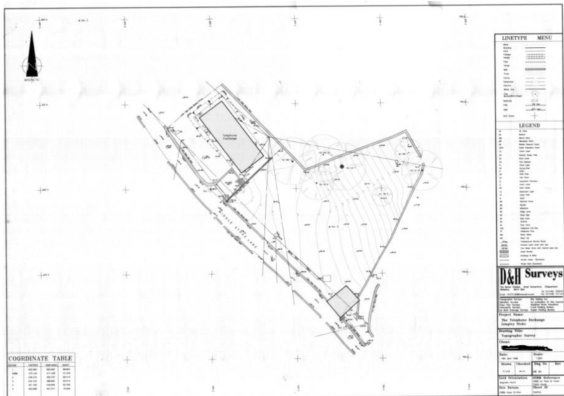
Figure 2. Topographical Survey
