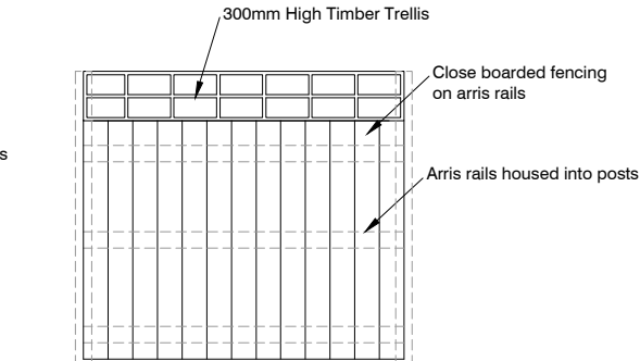
1.5m High Close Board Fence with 300mm Timber Trellis
