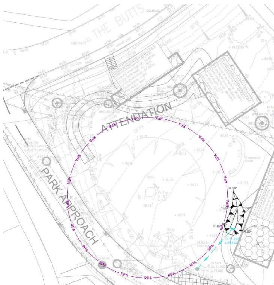
Figure 3.1 – Headwall relocation design proposal
