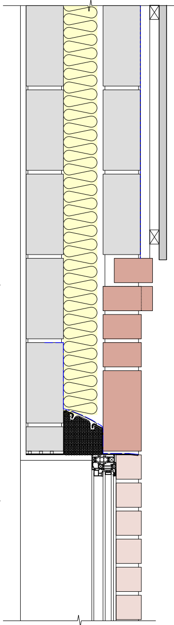
DET 04 Dentil Course 1:10
