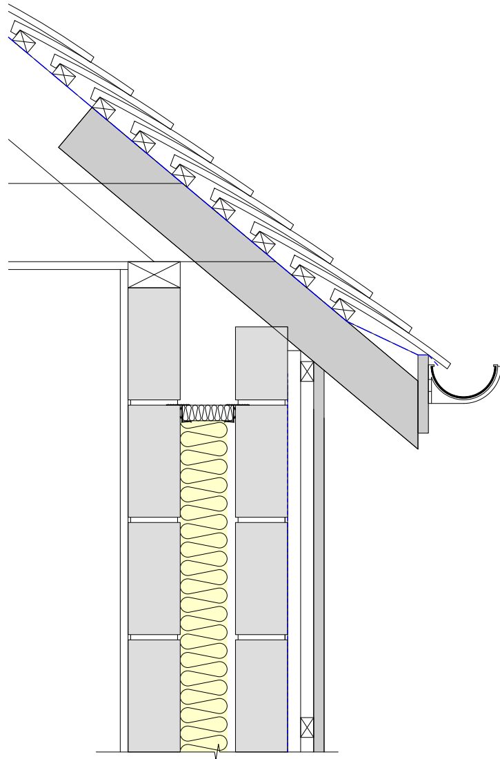
DET 01 Eaves Detail 01 1:10
