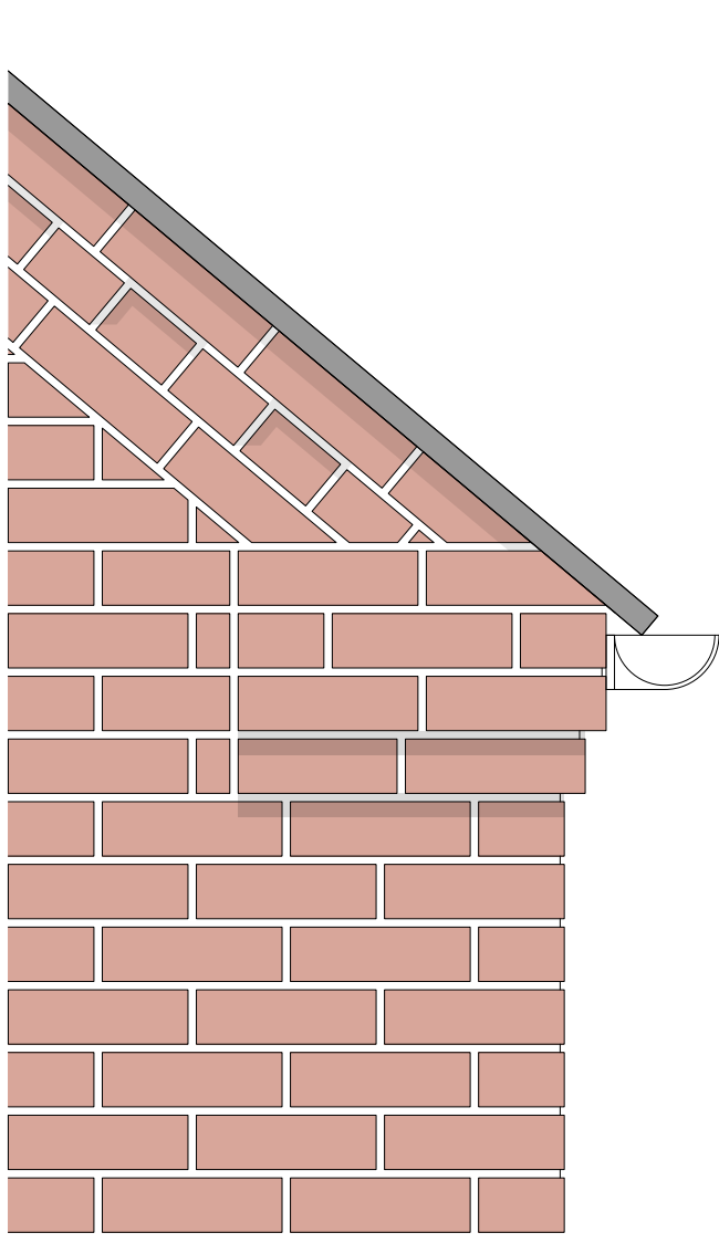
DET 03 Eaves Detail 03 1:10
