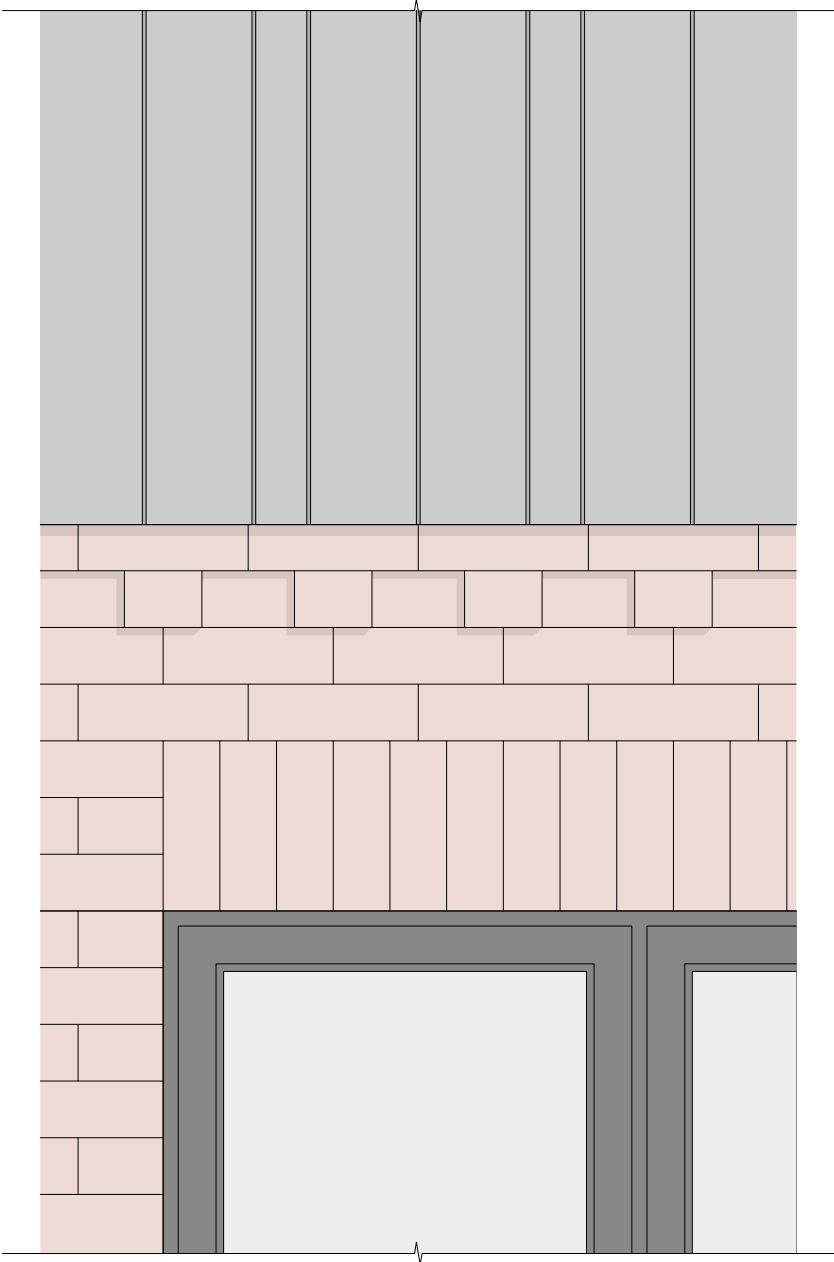
DET 06 Window Head 02 1:10
