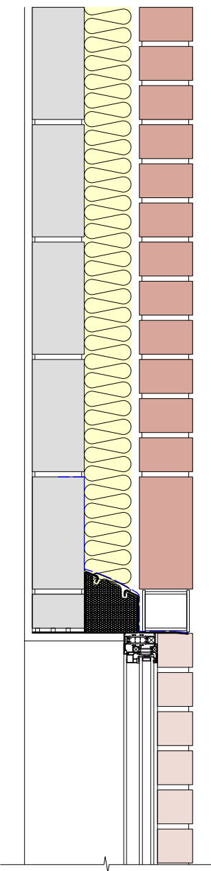
DET 06 Window Head 02 1:10
