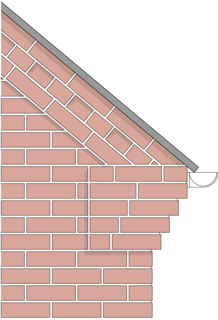
DET 02 Eaves Detail 02 1:10
