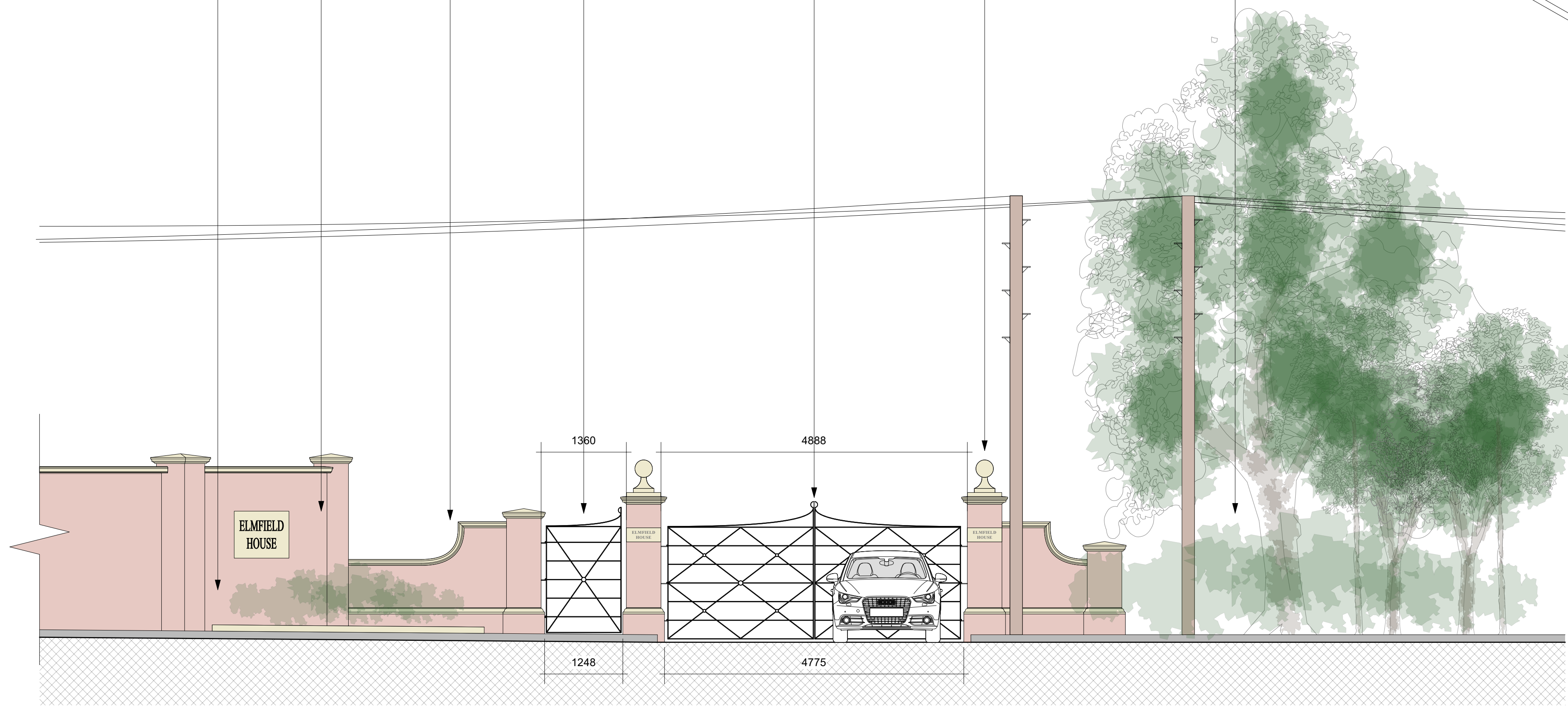
ELV 01 Proposed Entrance 1:50
