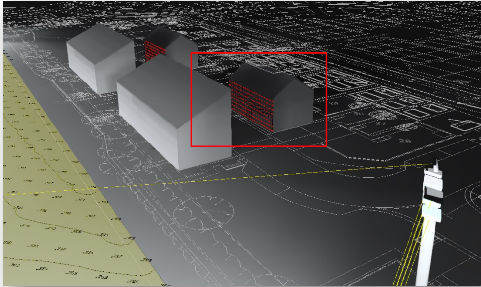
Figure 4.5: Plot 16 vertical calculation grid (shown in red)
