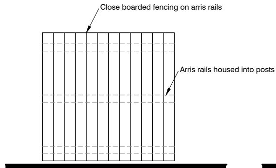
1.8m High Close Board Fence
