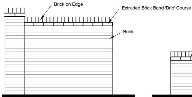
1m High Bin Screen Wall
