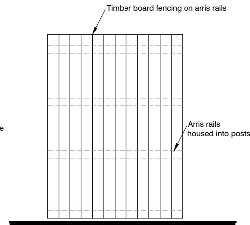
2.5m High Timber Acoustic Fence
