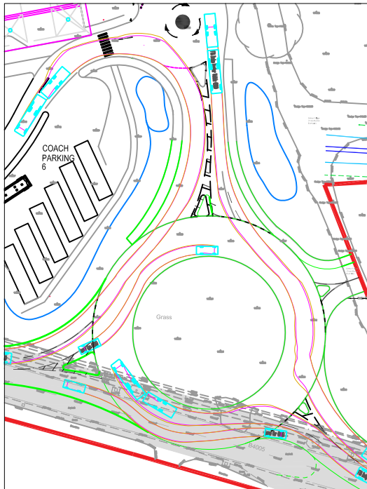
DRAWBAR VEHICLE
